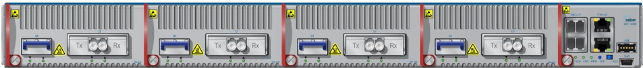
SABER-4400 with 4 TMX-4400 modules
